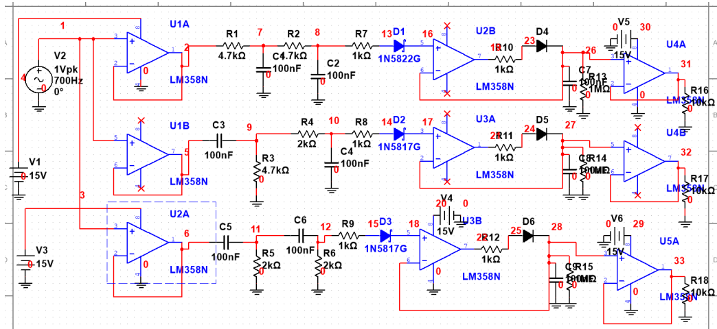
Figure 1: Circuit Diagram of Filters and Envelope Detector
